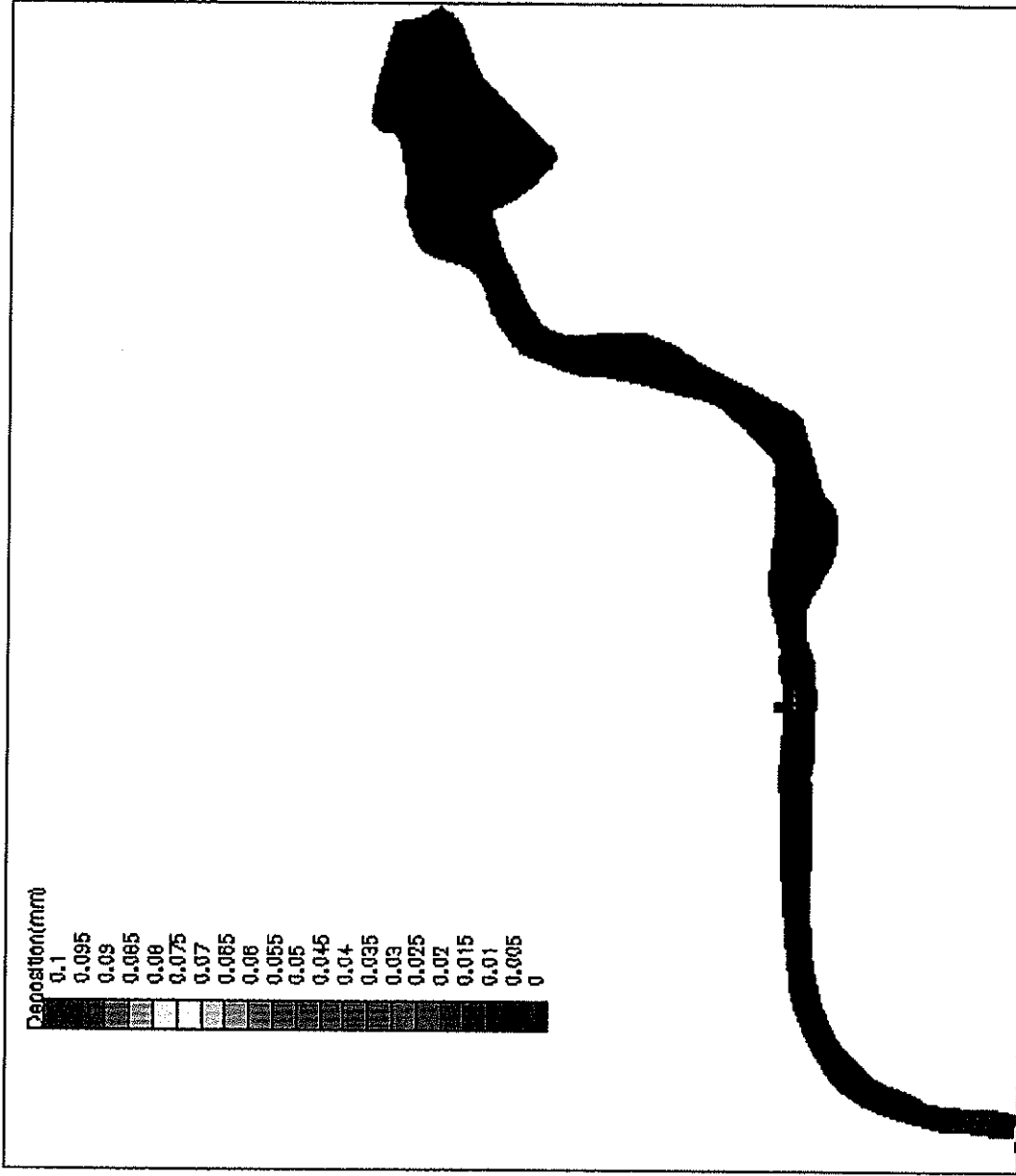
Figure F.1 Contours of Sediment Deposition for Fine Silt after Six Tidal Cycles (spring/middle)
