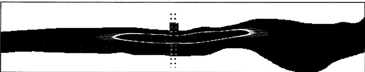
Figure F.17 Contours of Sediment Deposition for Medium Sand after Six Tidal Cycles (spring/middle)
