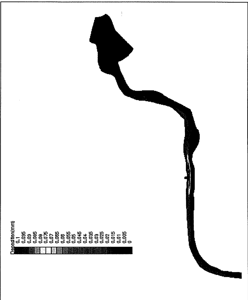
Figure F.5 Contours of Sediment Deposition for Coarse Silt after Six Tidal Cycles (spring/middle)
