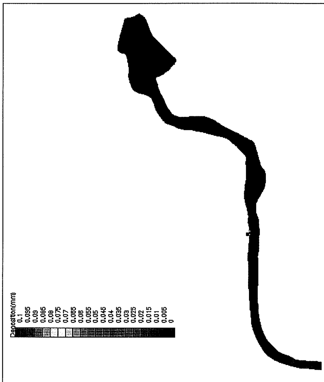
Figure F.2 Contours of Sediment Deposition for Fine Silt after Six Tidal Cycles (spring/north)
