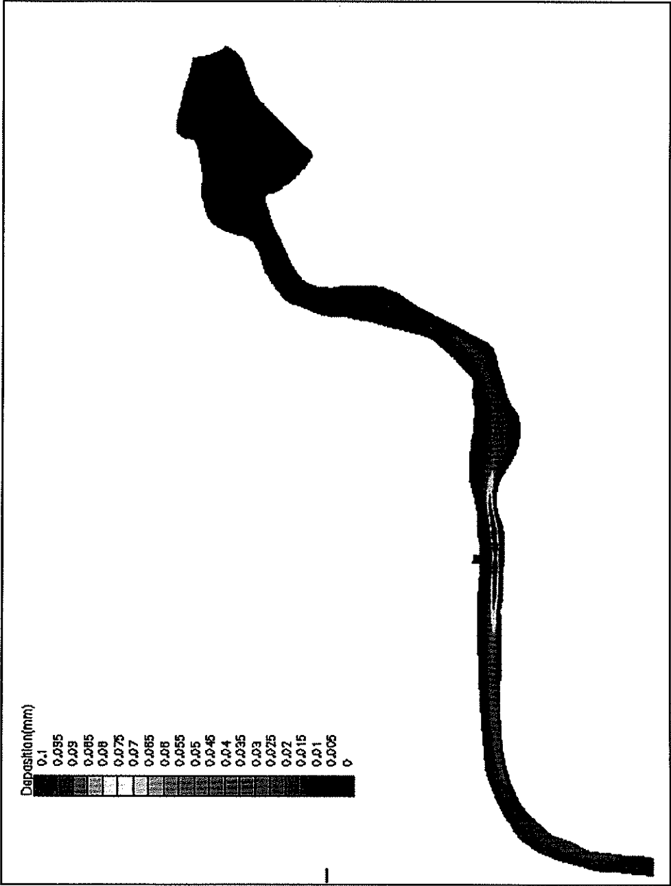
Figure F.7 Contours of Sediment Deposition for Coarse Silt after Six Tidal Cycles (spring/south)
