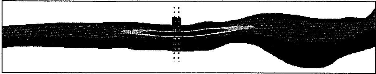
Figure F.14 Contours of Sediment Deposition for Coarse Silt after Six Tidal Cycles (spring/middle)
