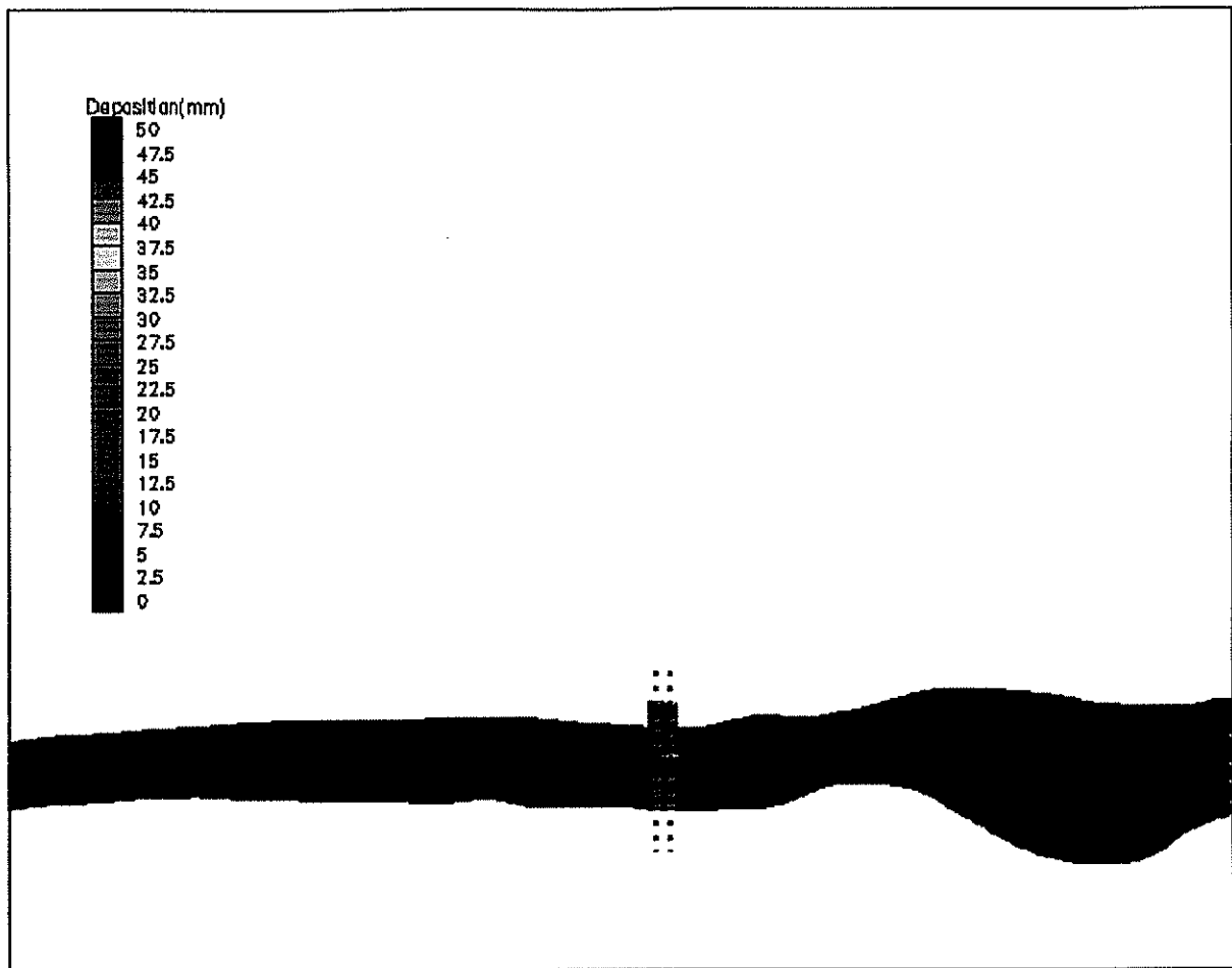
Figure F.18 Contours of Sediment Deposition for Medium Sand after Six Tidal Cycles (spring/middle)
