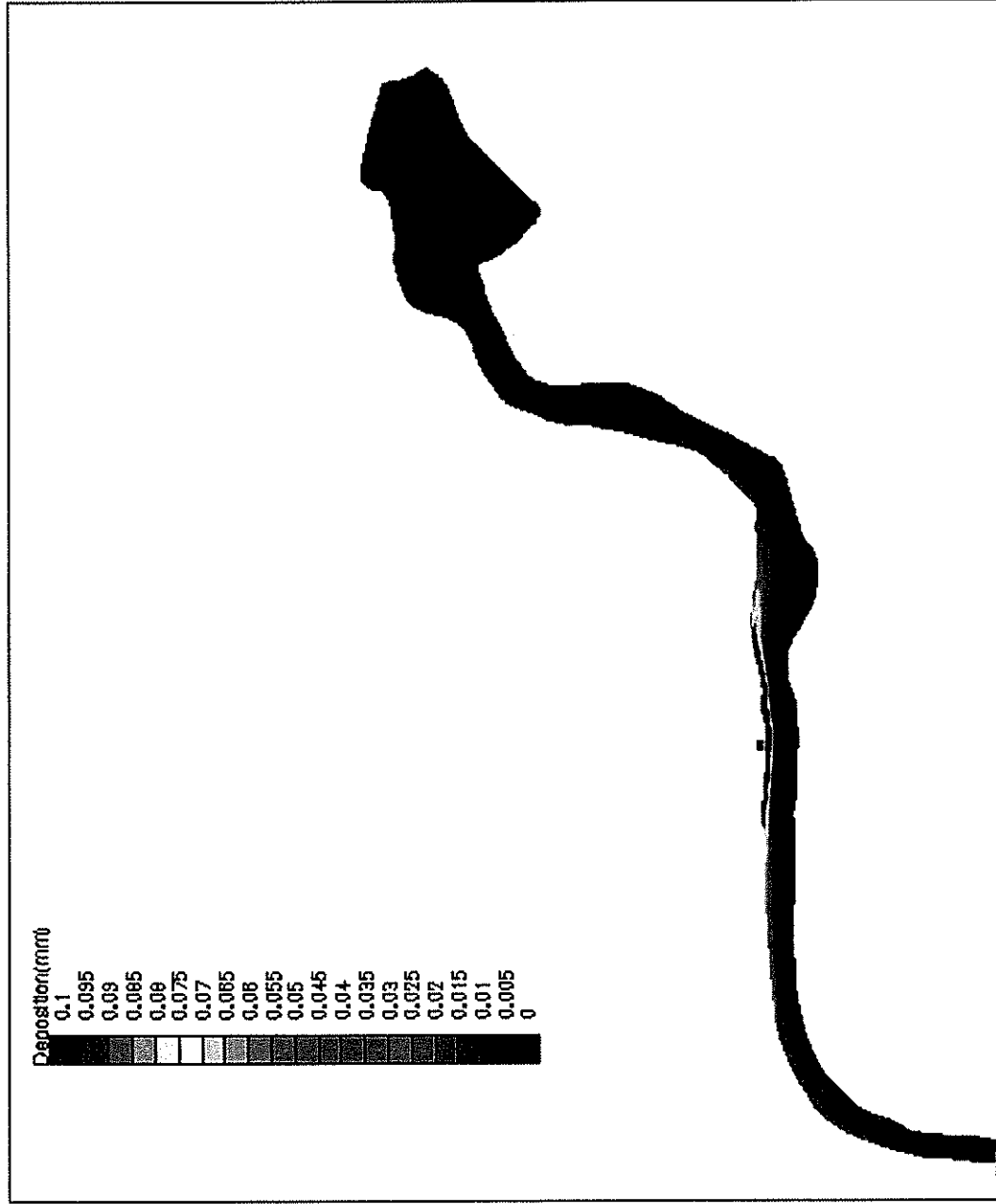
Figure F.6 Contours of Sediment Deposition for Coarse Silt after Six Tidal Cycles (spring/north)
