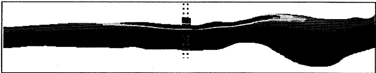
Figure F.15 Contours of Sediment Deposition for Coarse Silt after Six Tidal Cycles (spring/north)
