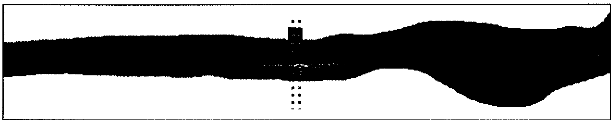
Figure F.12 Contours of Sediment Deposition for Fine Silt after Six Tidal Cycles (spring/south)
